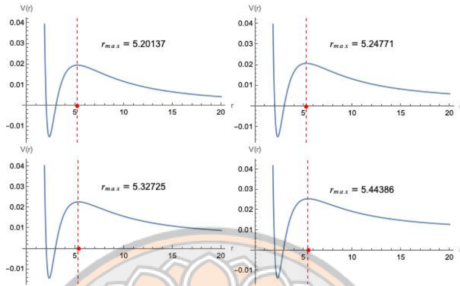
Figure 22 The effective potential of monopole mode and show the real value of r maximum of the peak.
