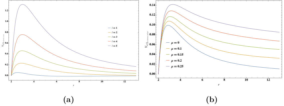
Figure 5 (a). The effective potential for the even-parity scalar modes with \omega = 0.4 , \mu = 0.1 , and variation l . (b). The effective potential for the even-parity scalar modes with \omega = 0.4 , l = 1 and variation \mu .
