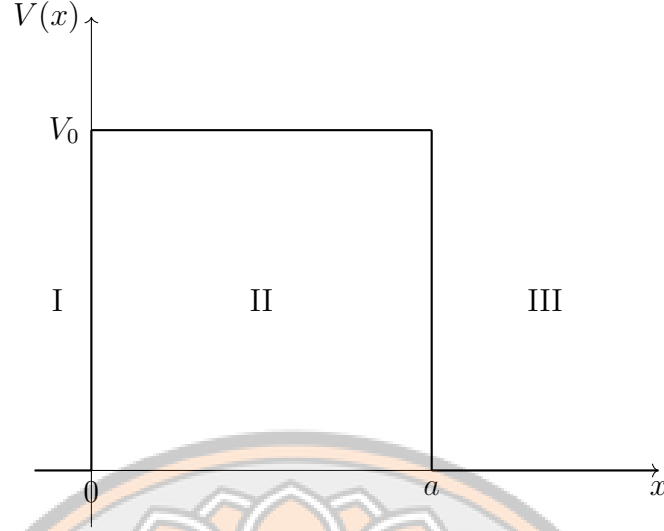
Figure 1 The barrier potential well.
