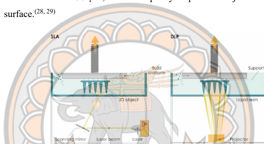
Figure 1 Schematic drawing of SLA and DLP printer
