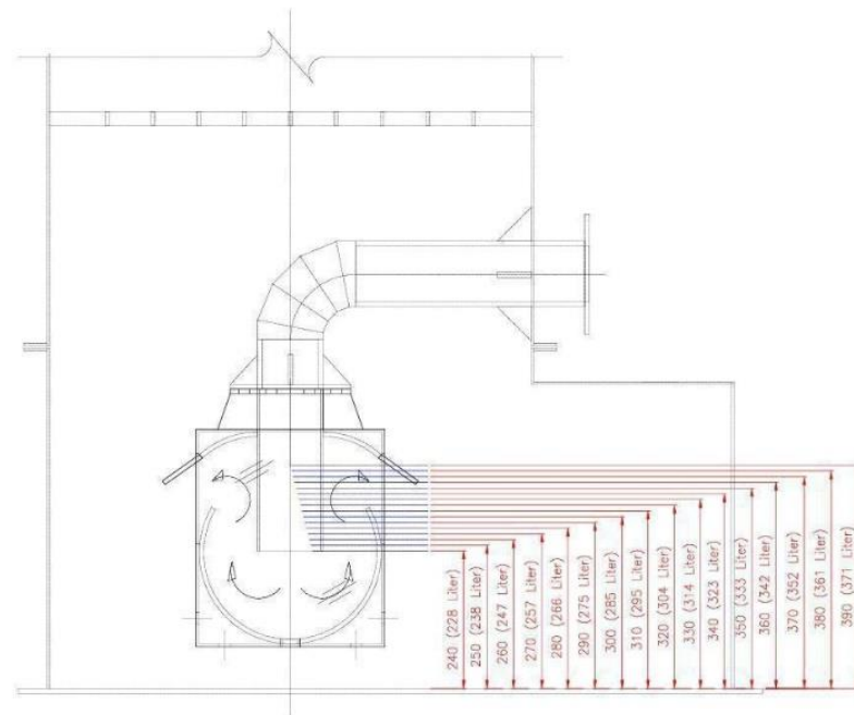
Figure 13 Integration of the Turbulence Water Box in the Wet Scrubber Tower
