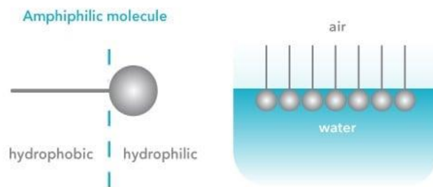
Figure 7 Surfactant's structure [31].
