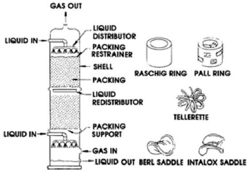
Figure 6 Packed bed scrubbers with some packing types retrieved [29]
