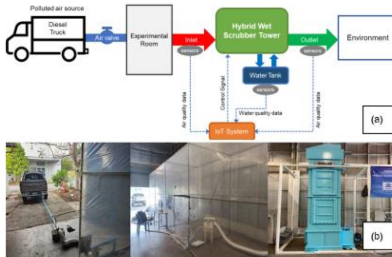
Figure 4 (a) Architecture diagram of the wet scrubber tower with an IoT system for an indoor experiment and (b) the developed wet scrubber tower installed in the indoor experimental room.
