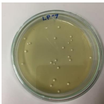
Lactobacillus plantarum
