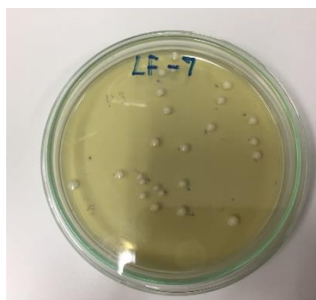
Lactobacillus fermentum
