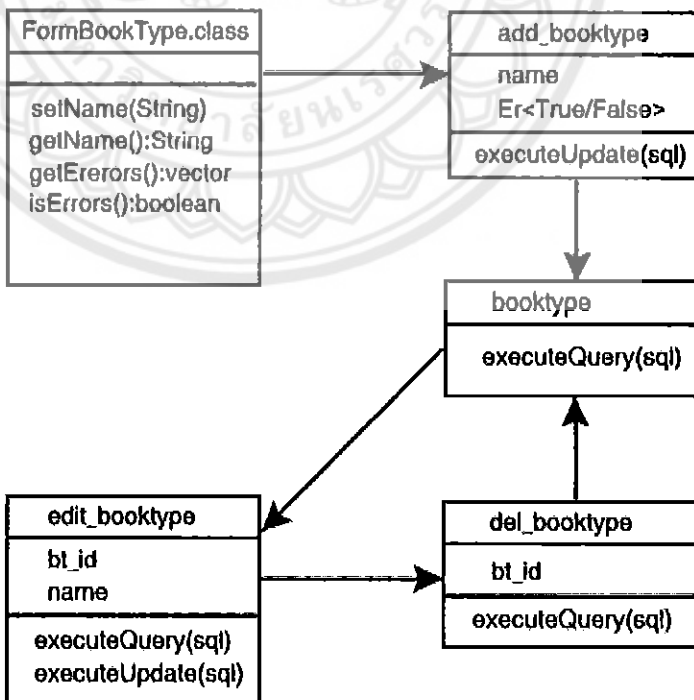
រូបភាព 3.12 Class Diagram : Booktype management
