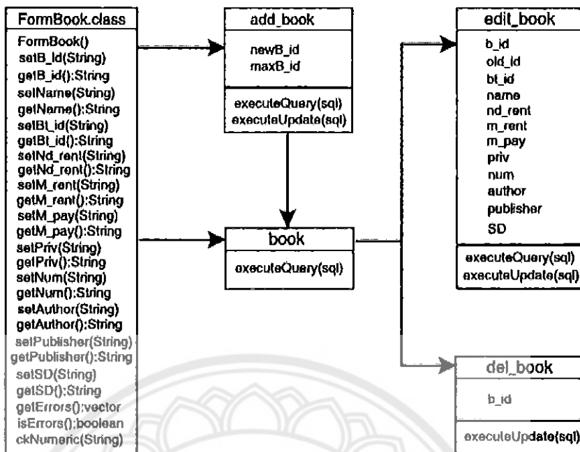
រូបភាព 3.11 Class Diagram : Book management
