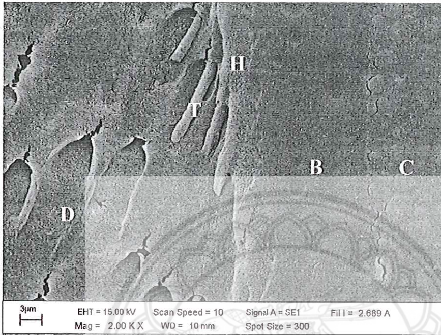
Figure 4: SEM photograph of the bonded interface between dentin cavity wall and adhesive system. Hybrid layer (H) and resin tags (T) can be seen. C: Resin composite. B: Bonding layer. D: Dentin.
